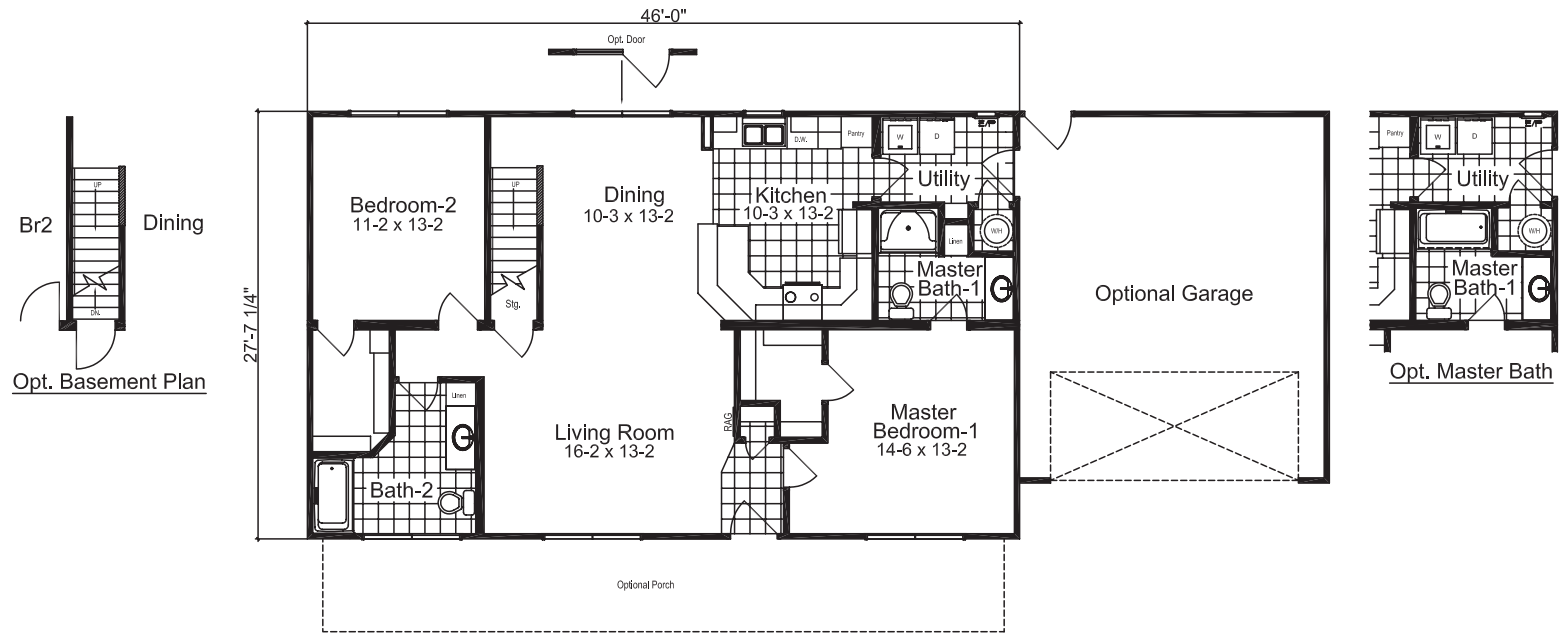
FIRST LEVEL FLOOR PLAN
